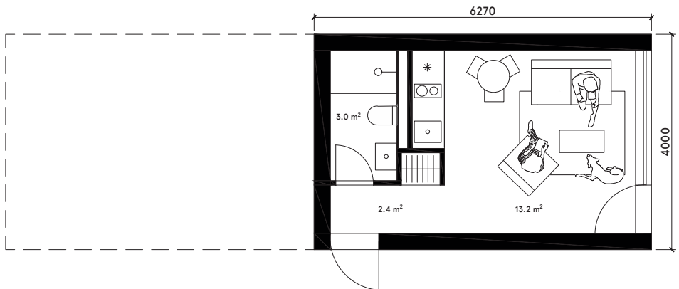
TYPE C Floor plans
